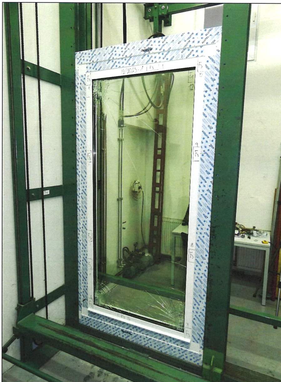
Pic. 8 – test sample No. 12/2023-1 after static tests
