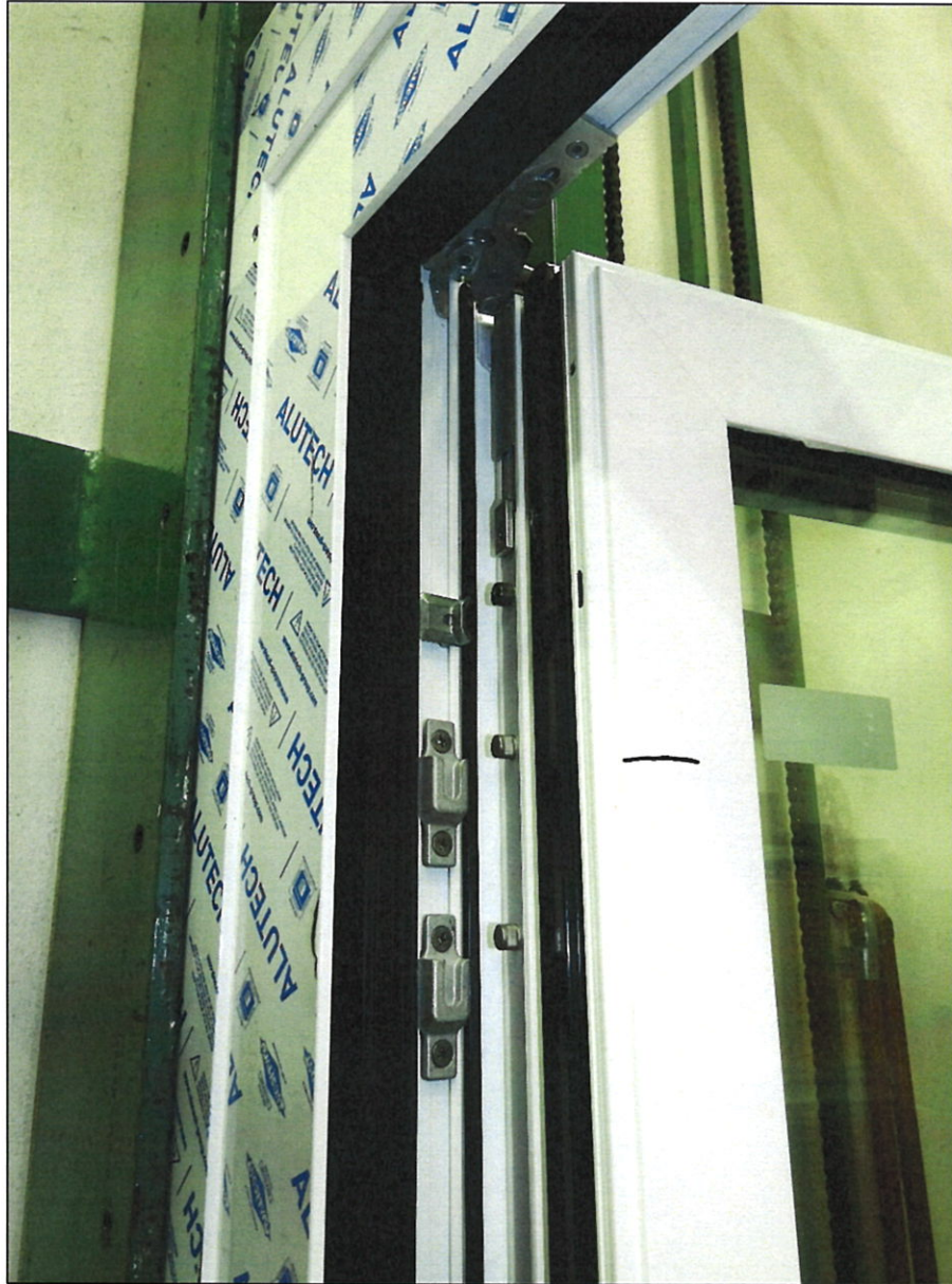
Pic. 3 – detail of upper hinge and locking pins
