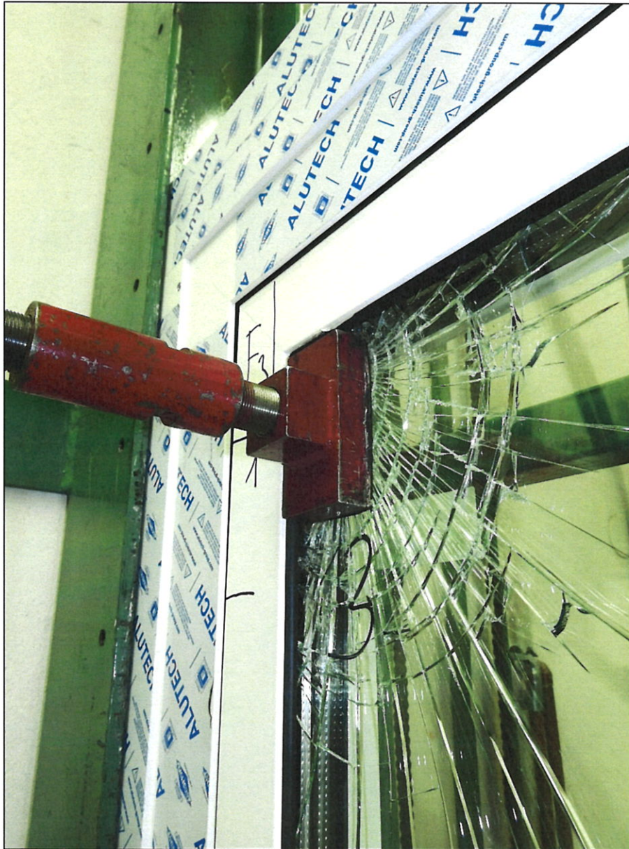
Pic. 7 – detail of point No. 13 during a static loading test, test sample No. 12/2023-1
